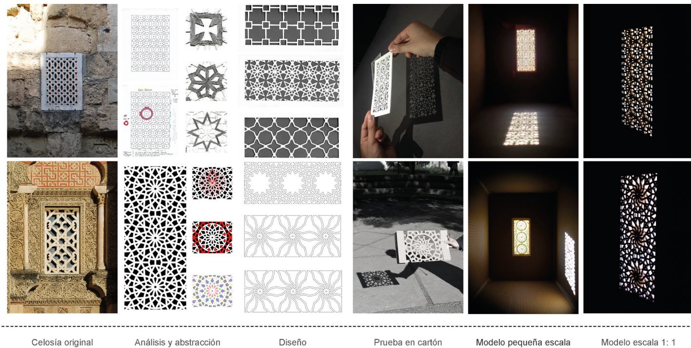
Figure 2: Summary of the process of analysis, design, and fabrication of a contemporary lattice inspired by a lattice from the Mosque of Córdoba I. (2019)
